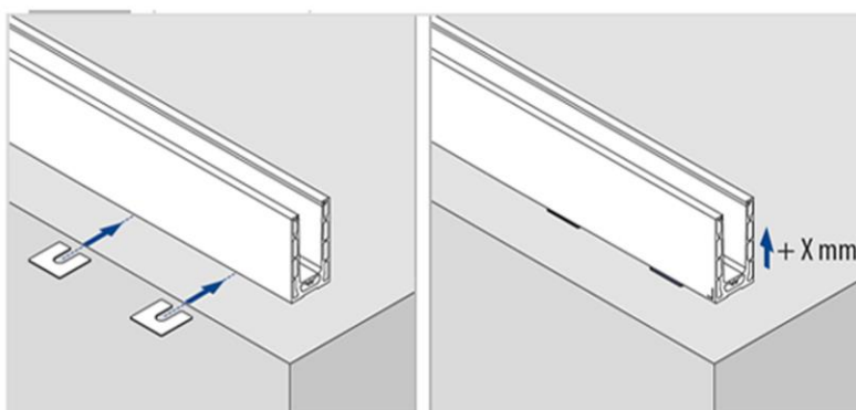
Shoe Shims for Easy Glass Smart Top Mount Base Channels (Pack of 100)
