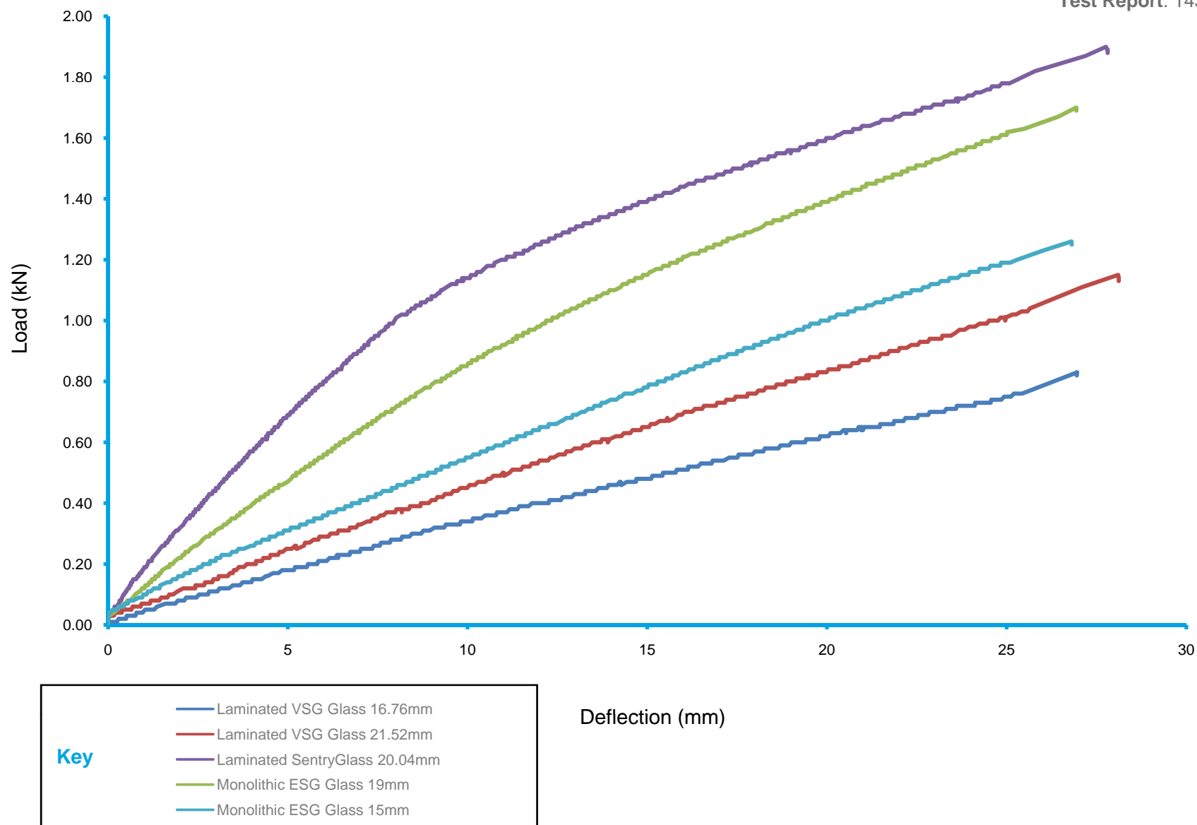
Chart 1: Load Versus Deflection Curves for Q-railing Easy Glass Pro Fascia Mount Fixed
