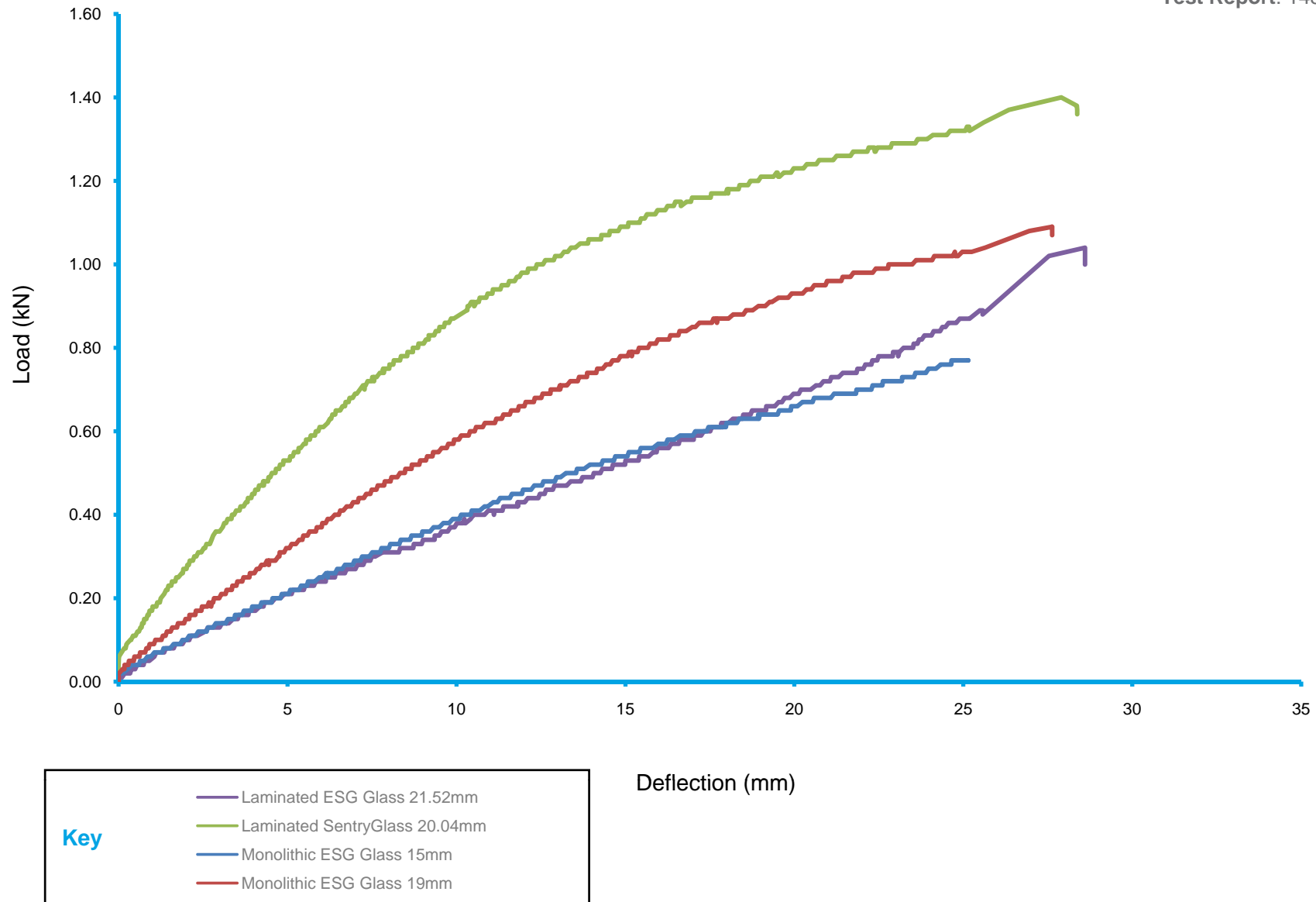
Chart 1: Load Versus Deflection Curves for Q-railing Easy Glass Pro Fascia Mount Adjustable
