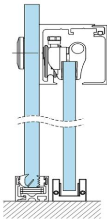
Sliding on Ceiling with Sidelight
