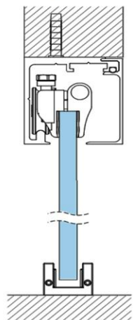
Sliding on Sidelight
