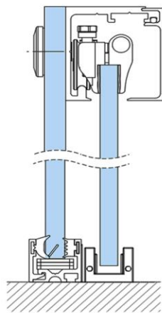
Installation with Supports on Wall
