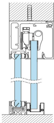
Sliding on Ceiling with Sidelight
