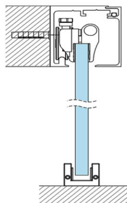
Installation with Supports on Wall
