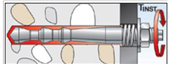
8. Allow to set, simply secure fixings using nut
