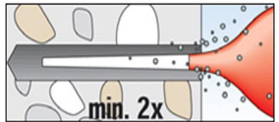
4. Clean again with air pump to achieve the perfect fixing surface.
