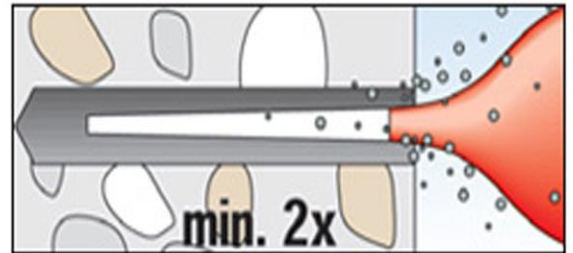
2. Clean with air pump to remove dust and debris.
